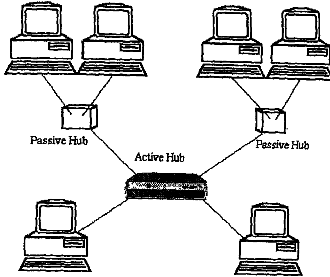
ARCNET Architecture
